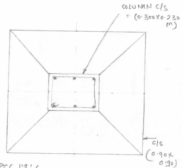
FOOTING PLAN.
